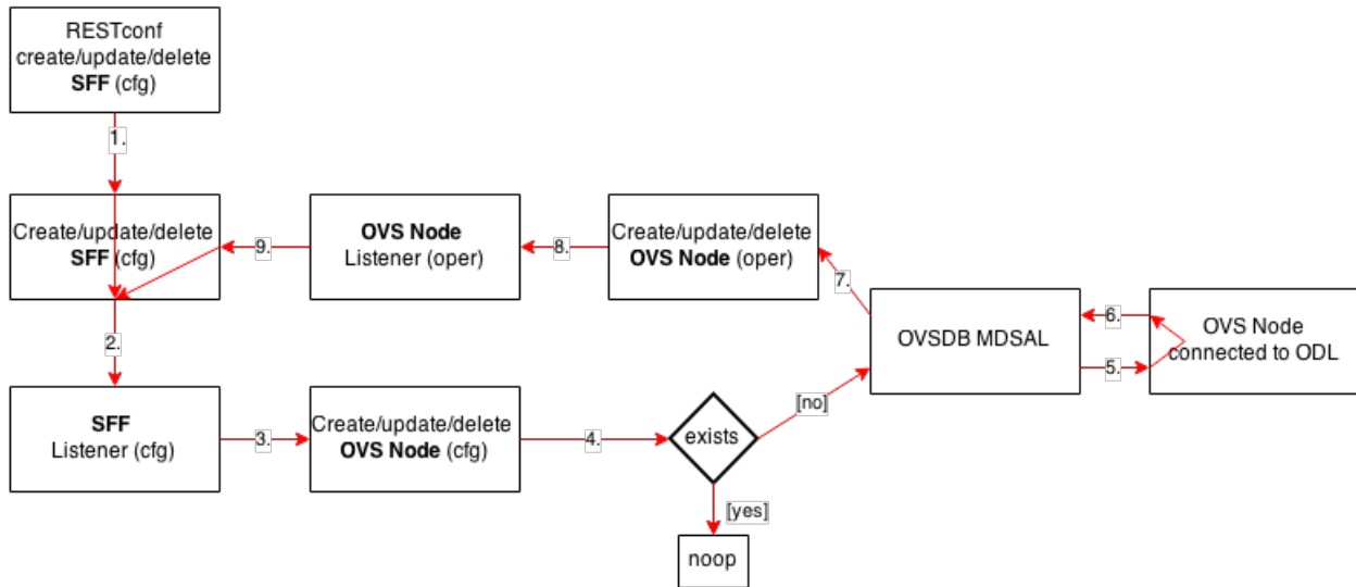
Fig. 1: SFC <—> OVS mapping flow diagram
