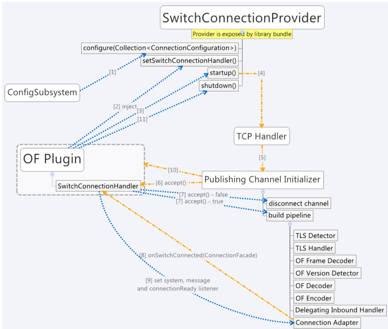
Fig. 7: Library lifecycle
