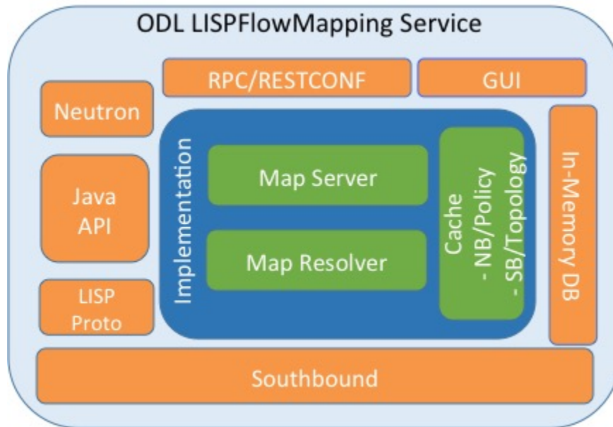
Fig. 1: LISP Mapping Service Internal Architecture
