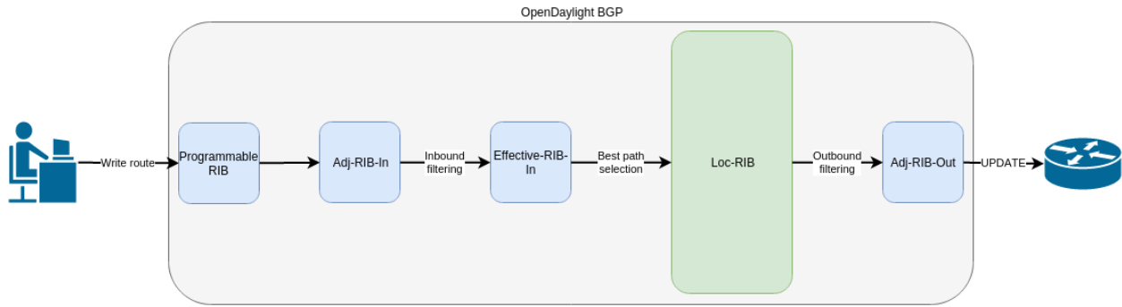
Fig. 1.22: BGP application peer pipeline - routes injection.
