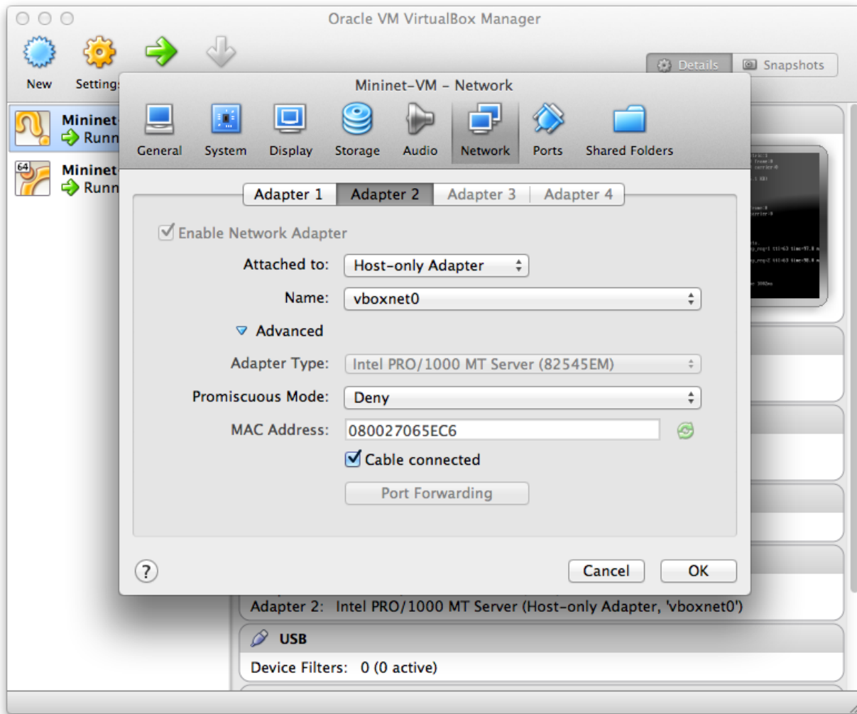
Fig. 1.81: configuring a host-only adapter
