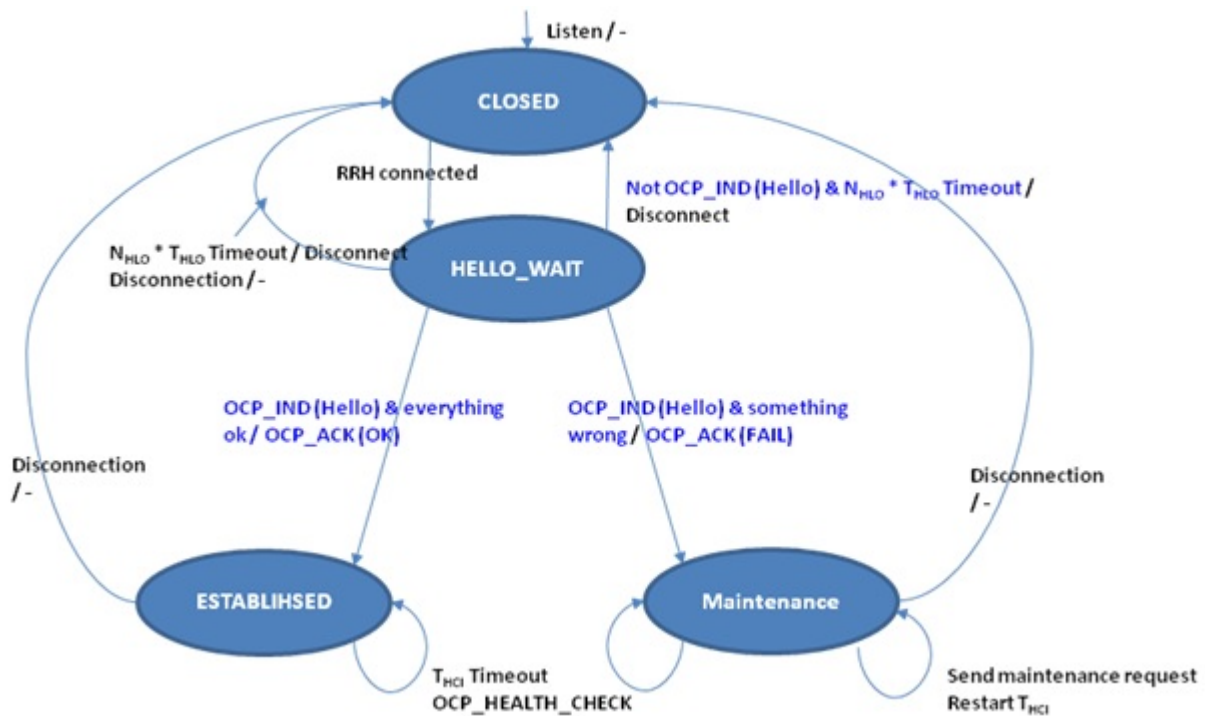
Fig. 2.27: OCP plugin state machine
