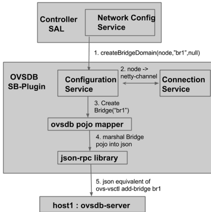
Fig. 2.38: End-to-end handling of a Create Bridge request
