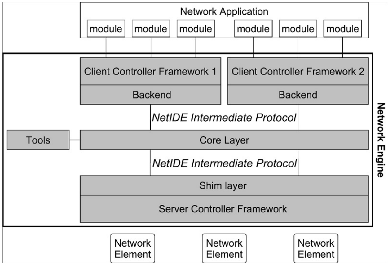
Fig. 2.22: NetIDE Network Engine Architecture
