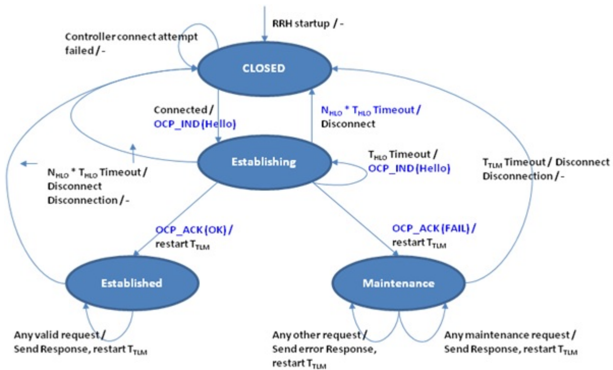
Fig. 2.26: OCP agent state machine
