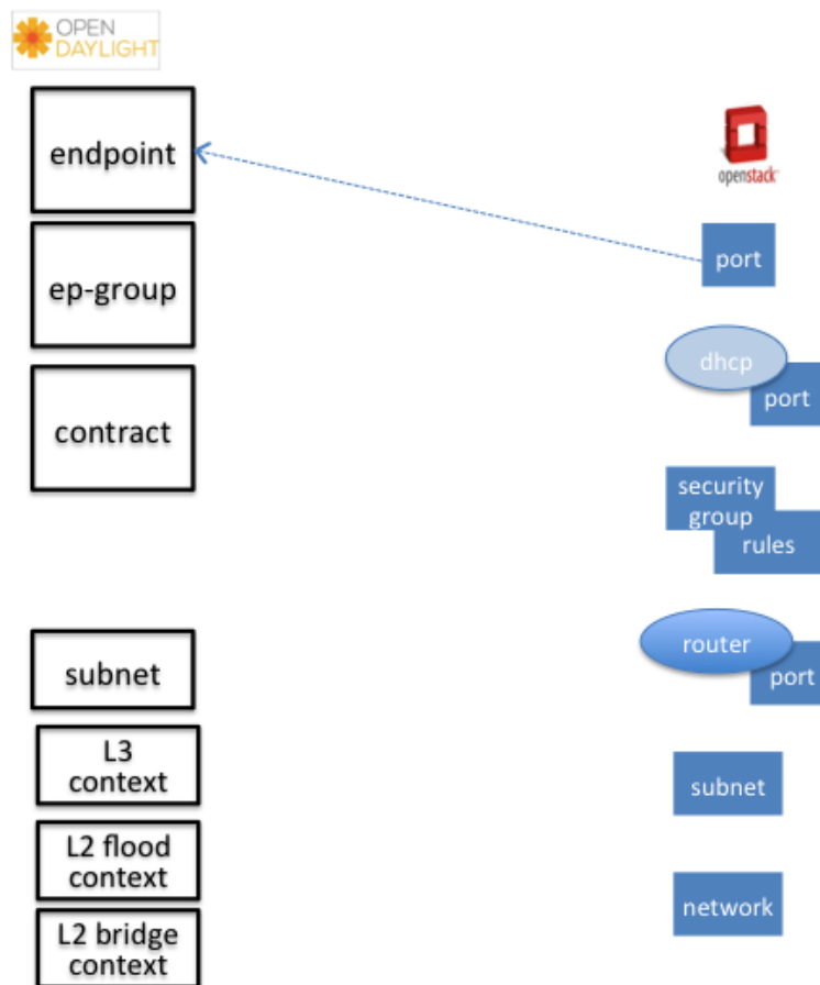
Fig. 1.51: Neutron Port
