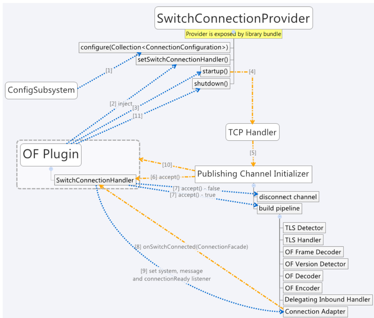
Fig. 2.30: Library lifecycle
