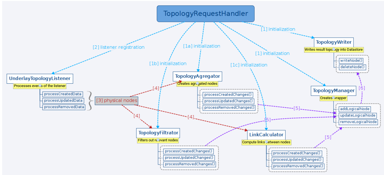
Fig. 2.59: Class relationship
