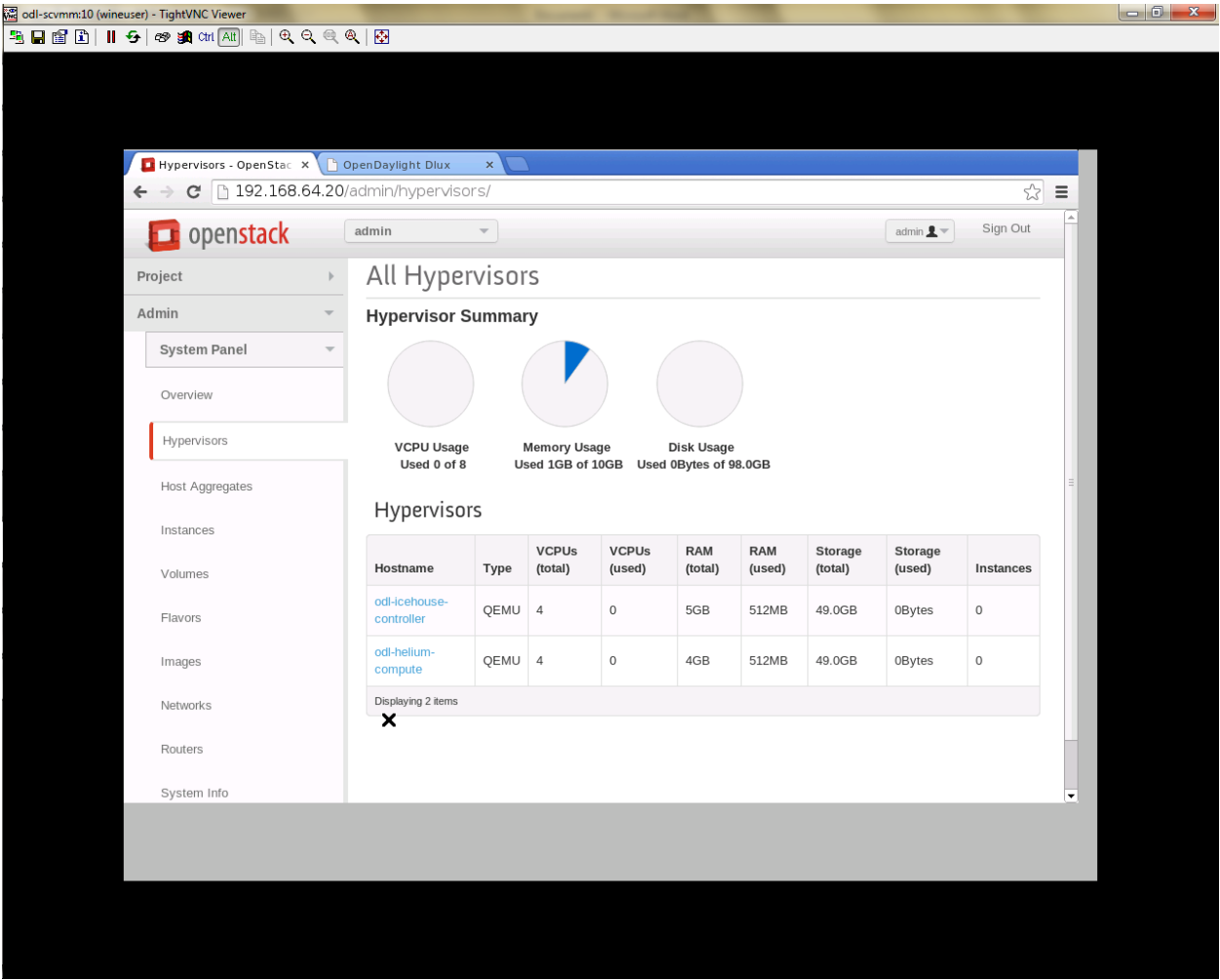
Fig. 1.121: Hypervisors
