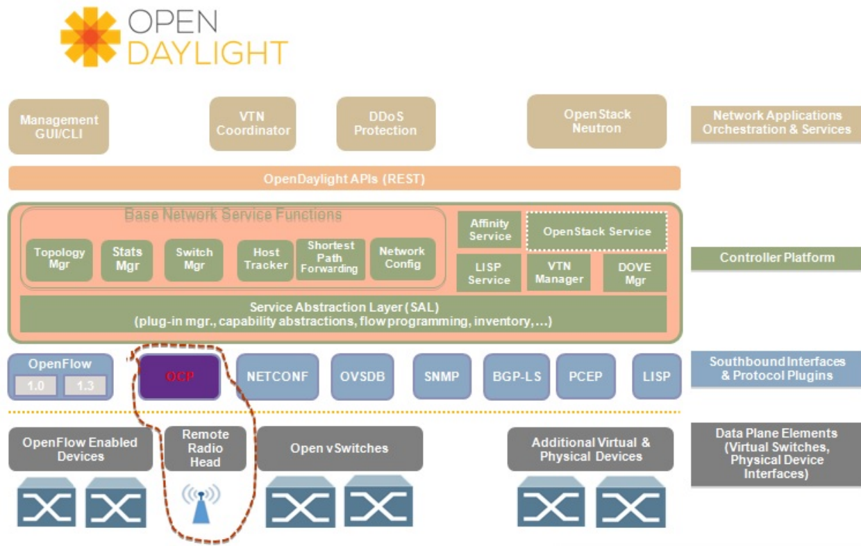
Fig. 2.24: OCP southbound plugin
