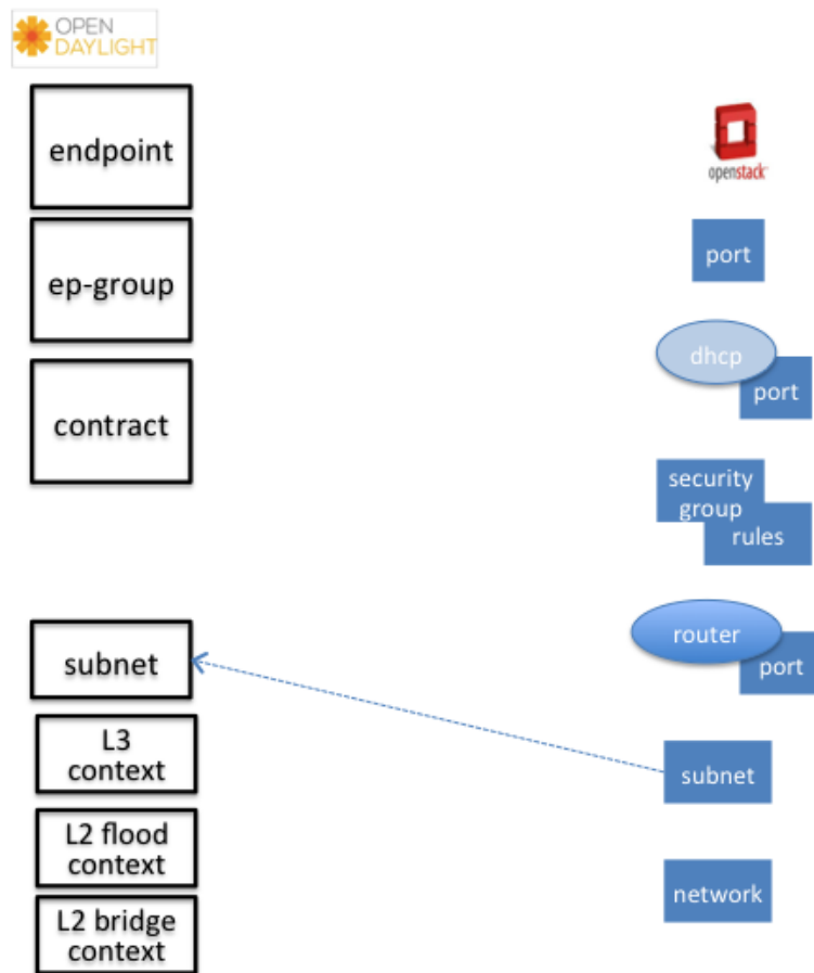
Fig. 1.155: Neutron Subnet
