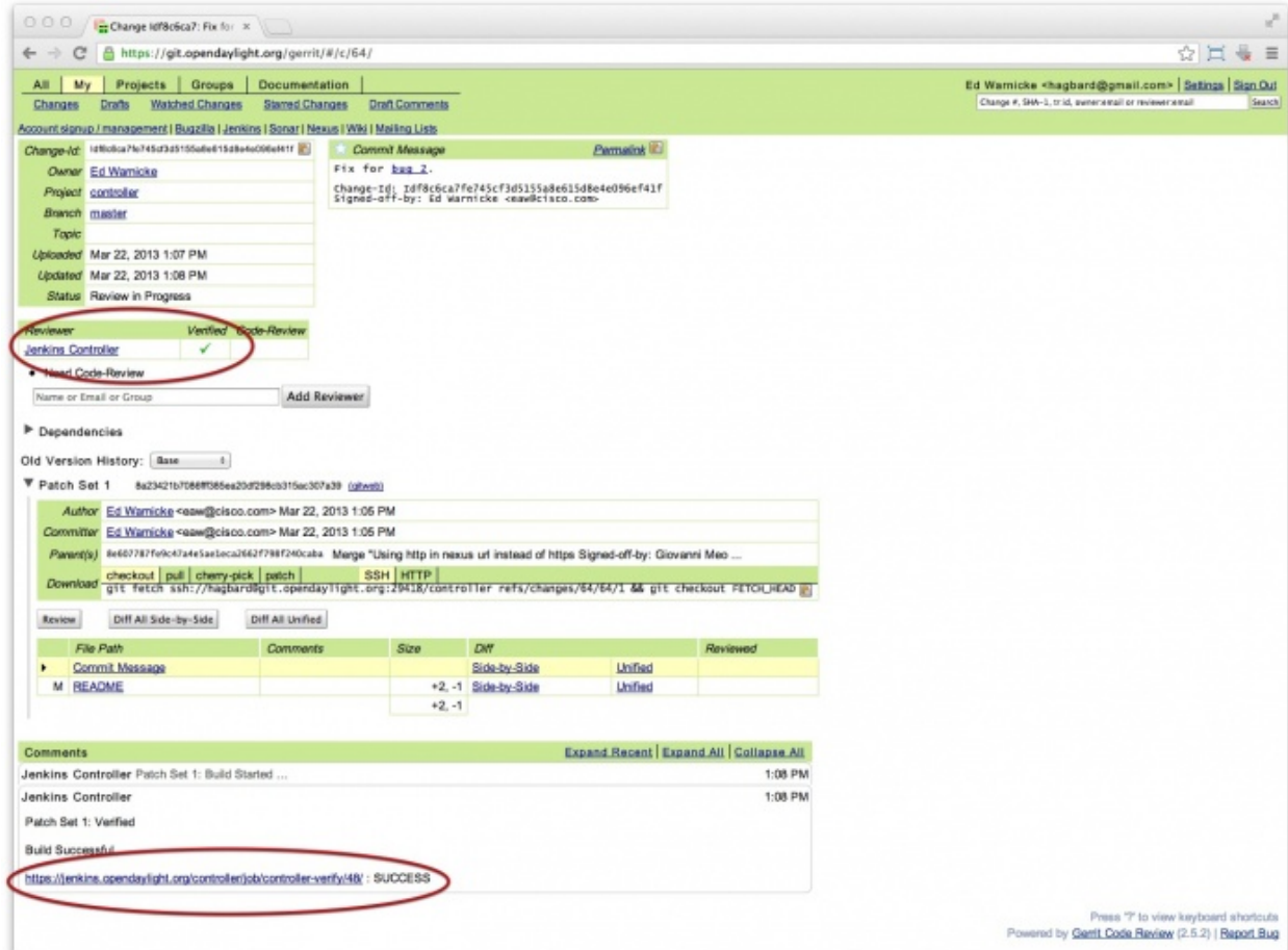
Fig. 2.10: Gerrit Code Review Sample
