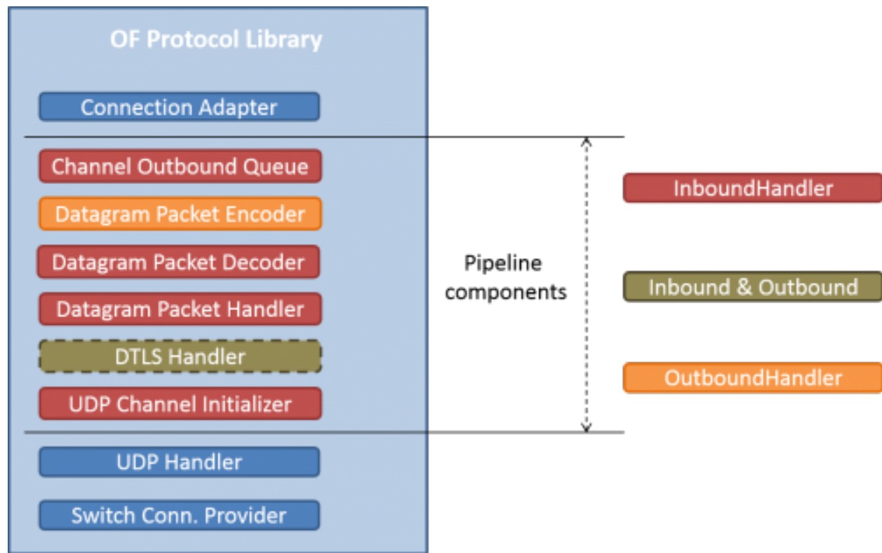
Fig. 2.29: UDP Channel pipeline
