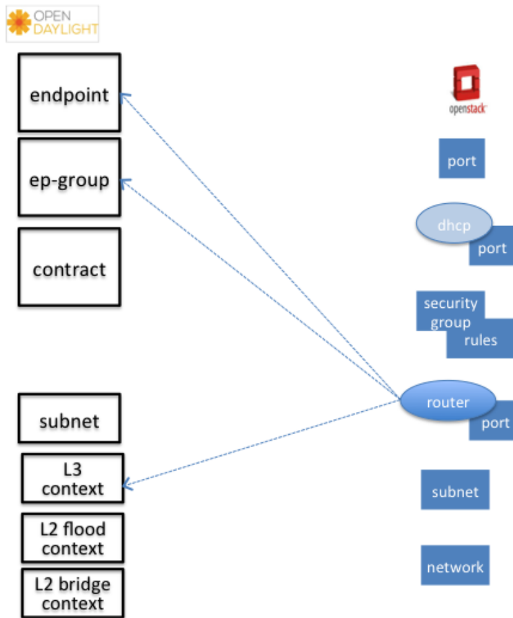
Fig. 1.157: Neutron Router
