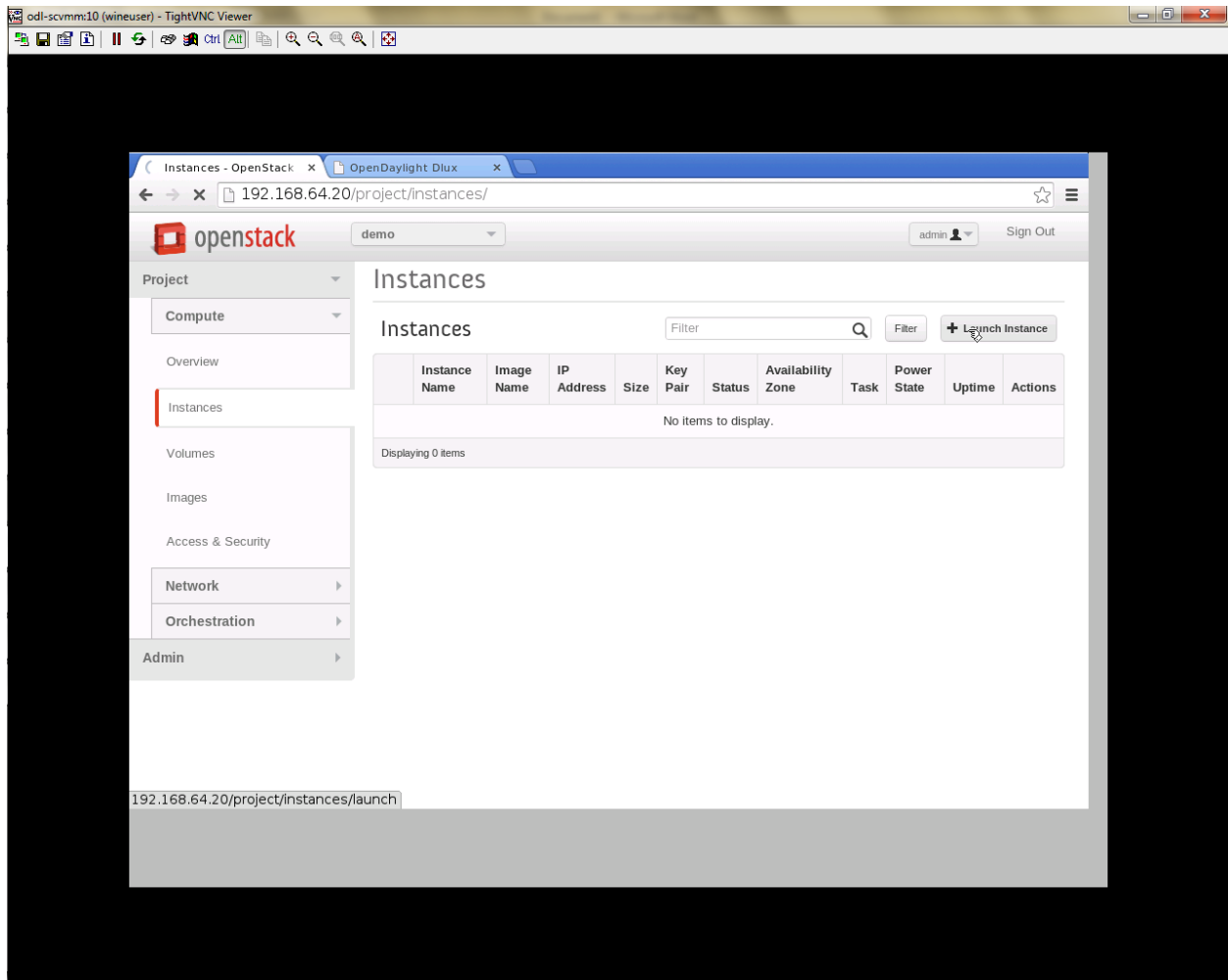
Fig. 1.126: Instance Creation
