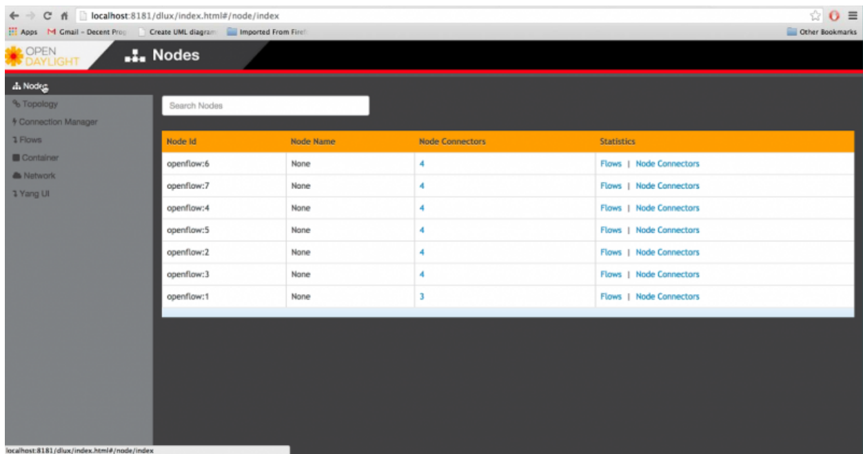
Fig. 1.132: DLUX_GUI
