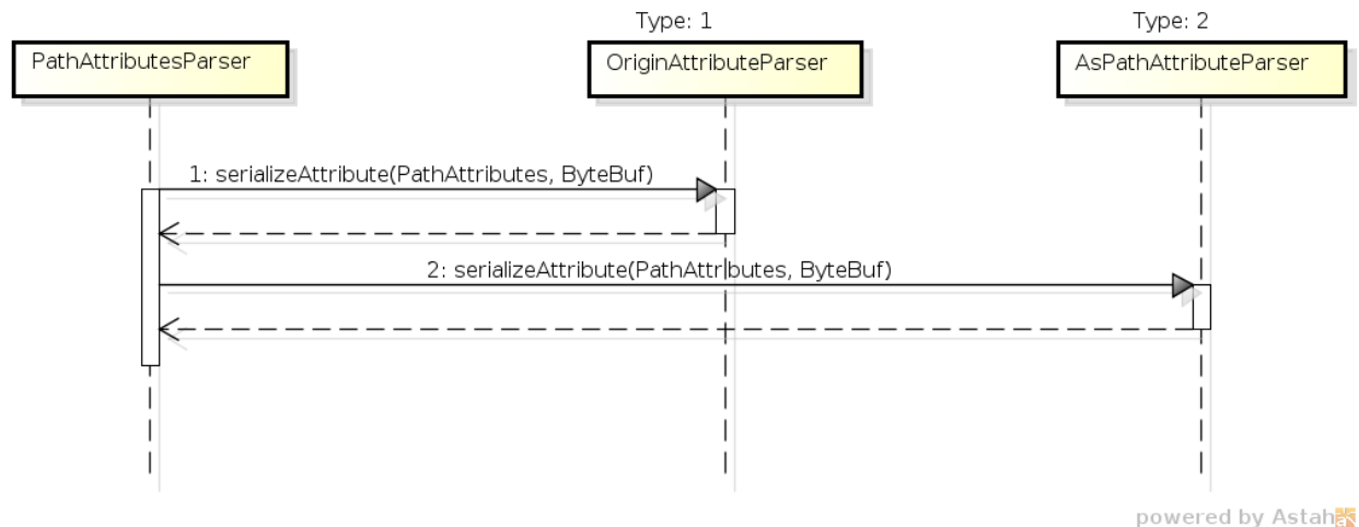
Fig. 2.15: PathAttributesSerialization
