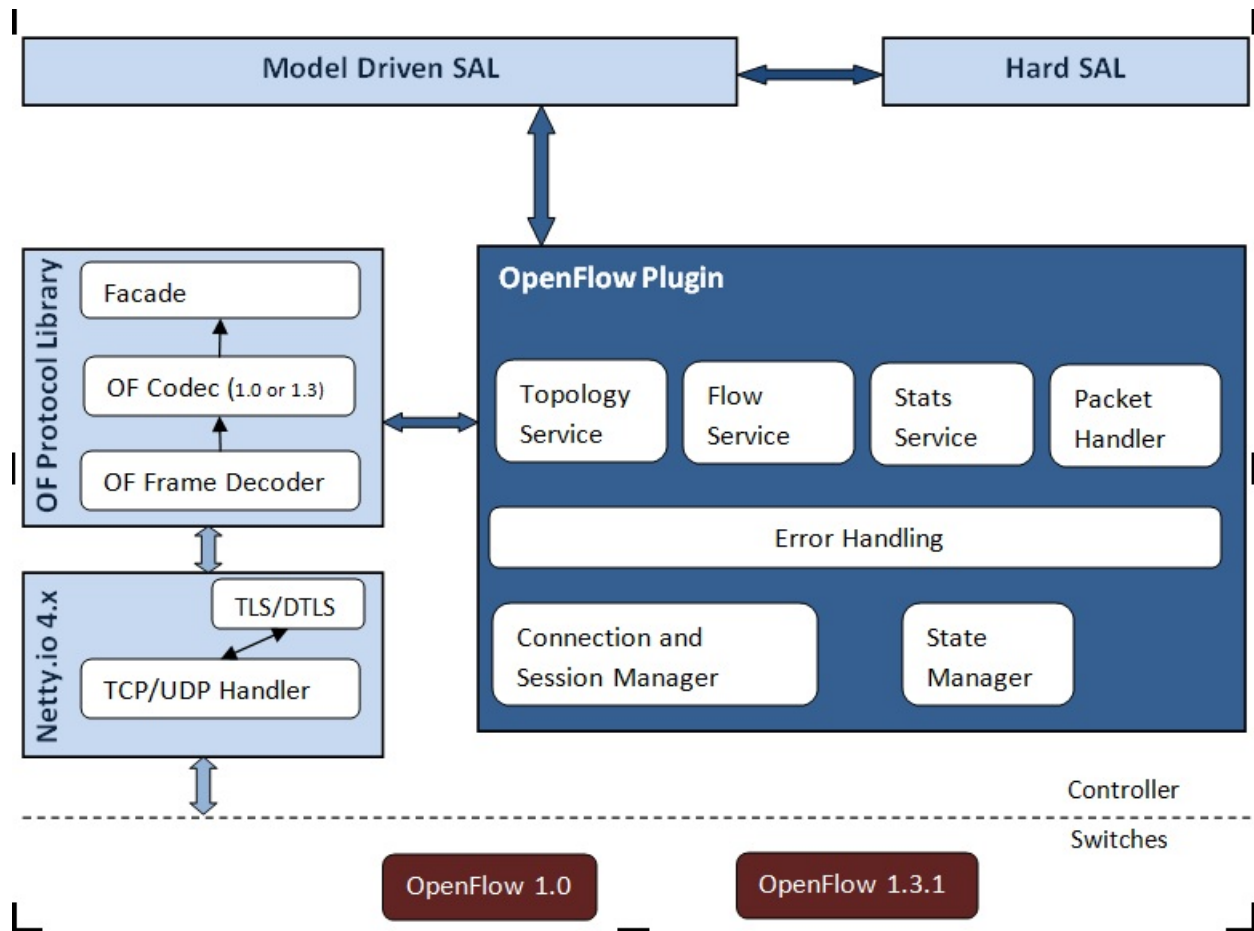
Fig. 1.80: overall architecture
