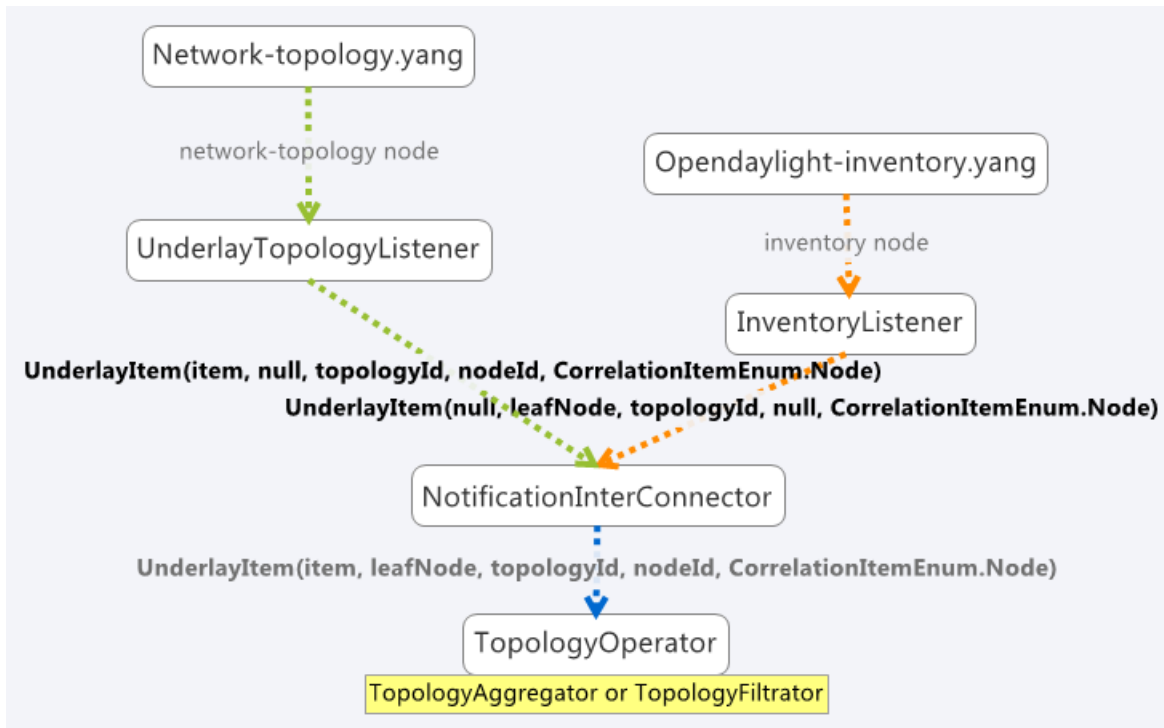
Fig. 2.62: Inventory model
