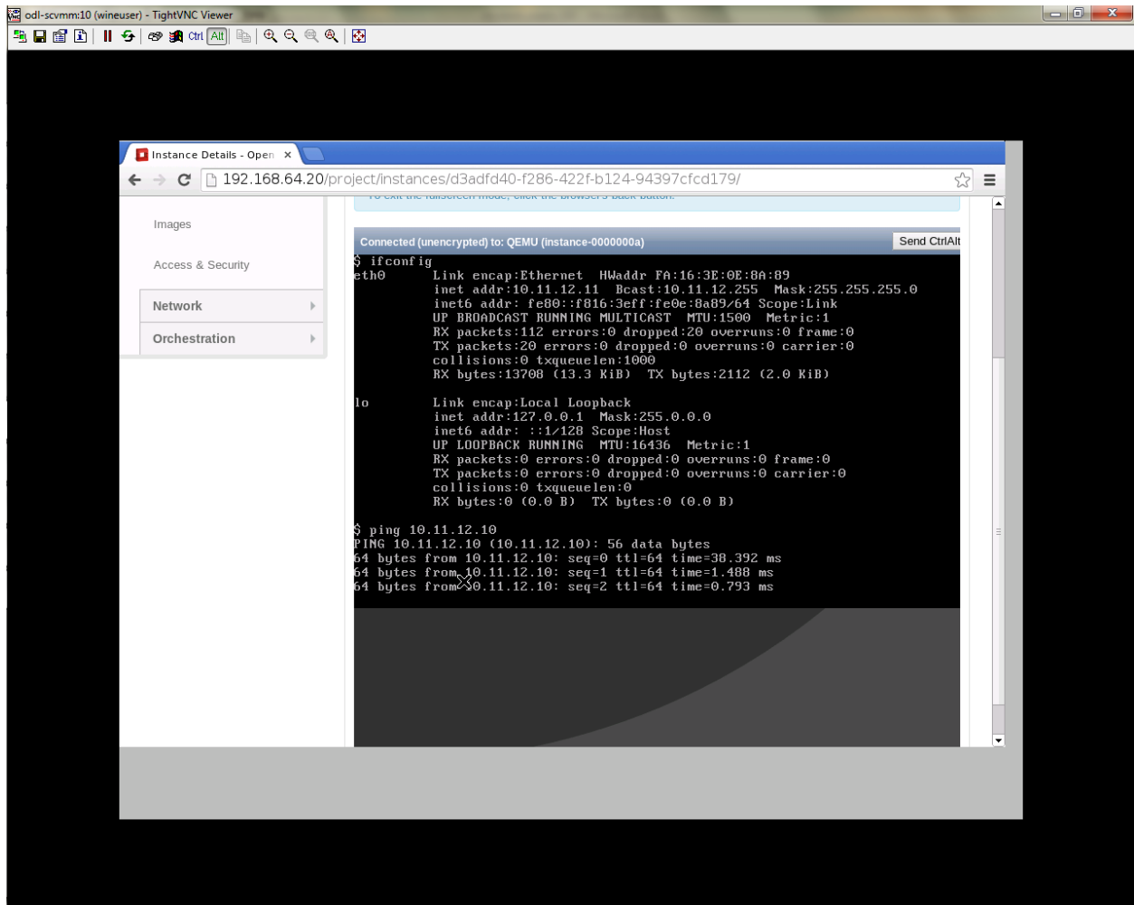
Fig. 1.131: Ping
