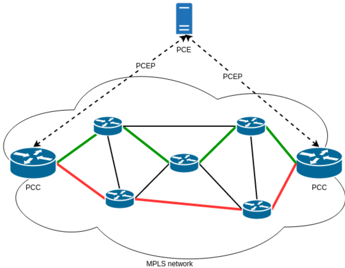
Fig. 1.82: PCE-based architecture.
