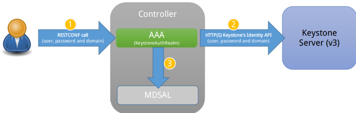
Fig. 2.13: KeystoneAuthRealm authentication/authorization mechanism
