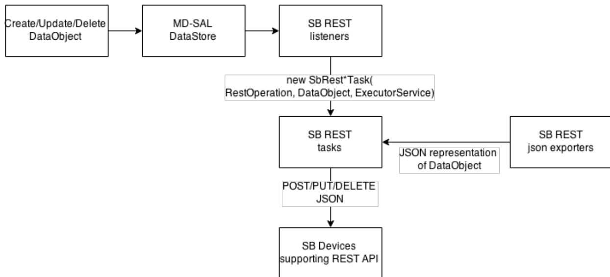
Fig. 2.49: Southbound REST Plug-in Architecture diagram
