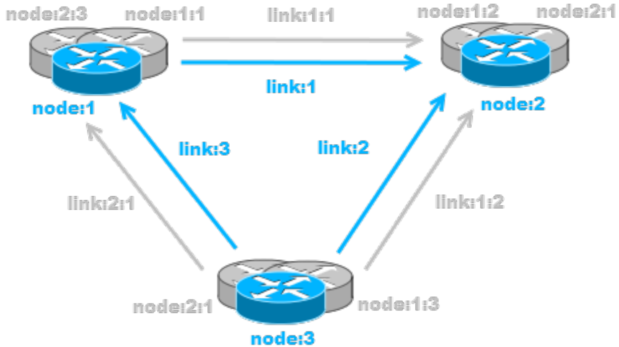
Fig. 2.63: Overlay topology with computed links
