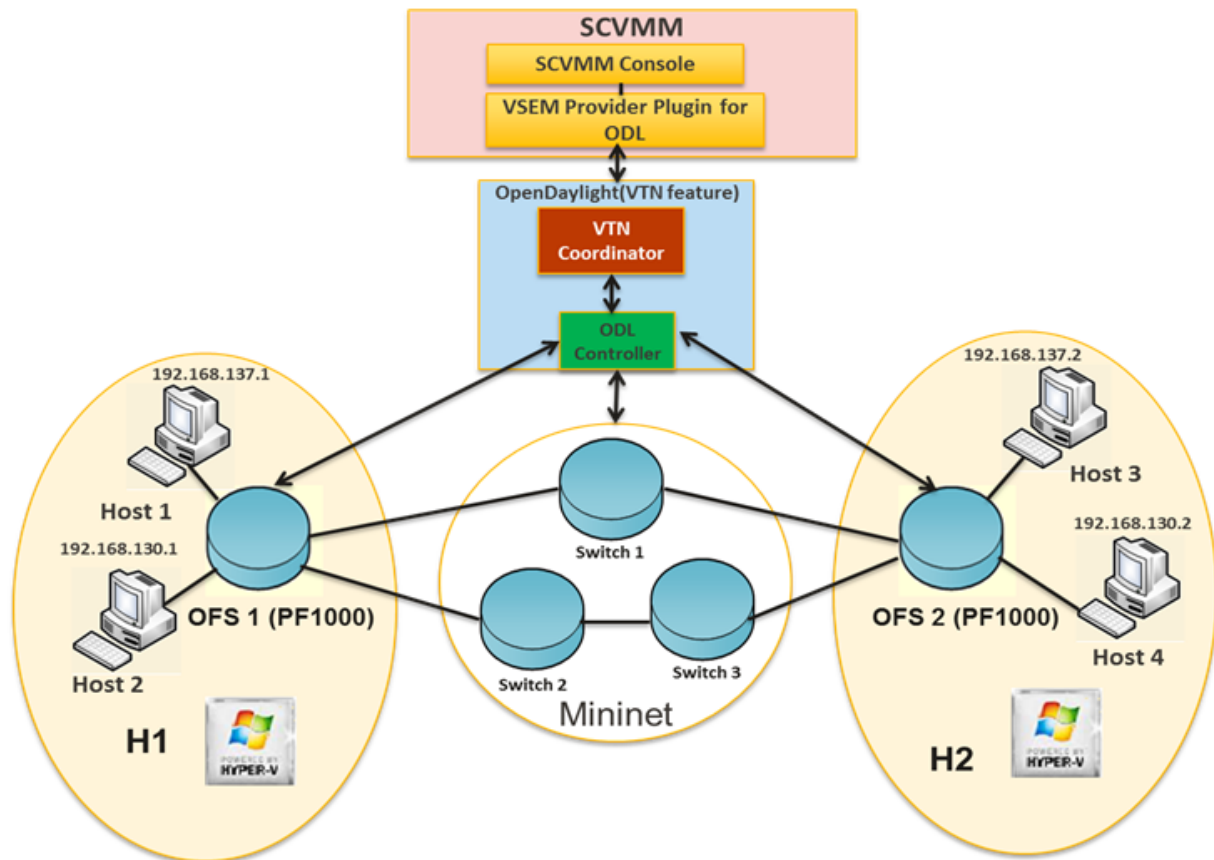
Fig. 1.152: Set-Up Diagram
