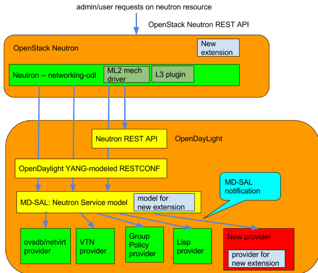
Fig. 2.23: Neutron Service Architecture
